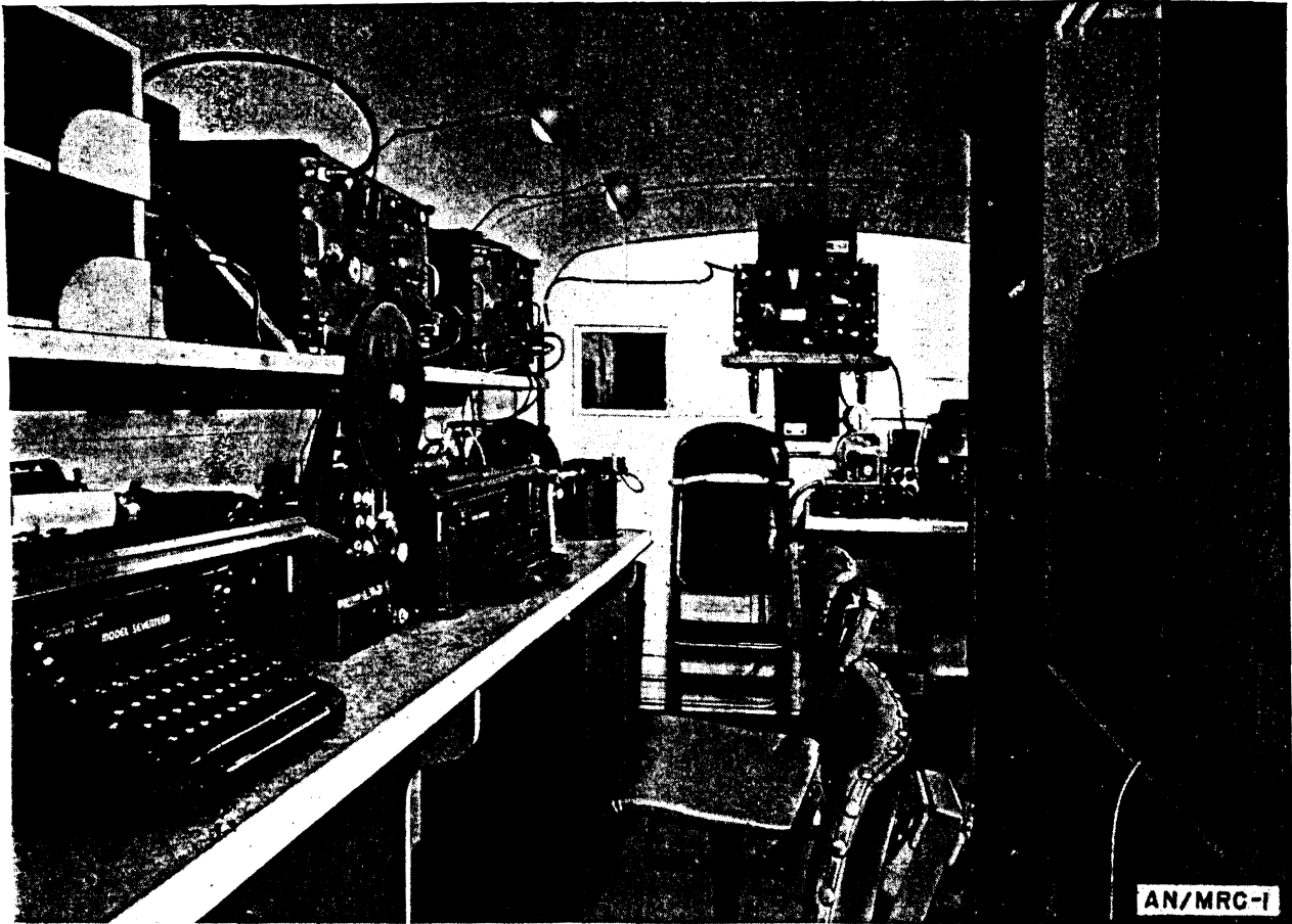
Figure 11. Radio Set AN/MRC-1, components installed in shelter.
