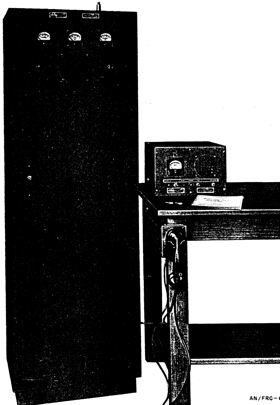
Figure 2. Radio Set AN/FRC-6.
